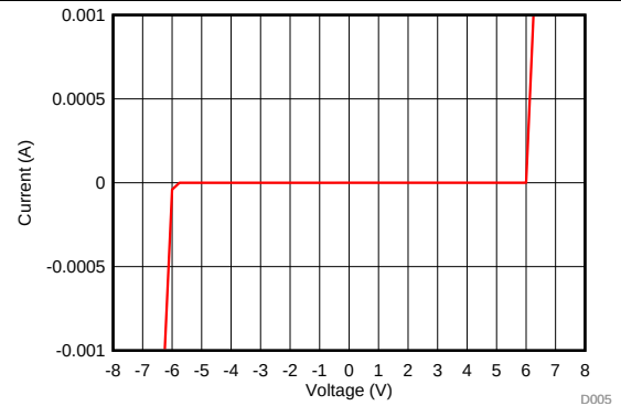
图 8. DC Voltage Sweep I-V Curve, IO pin to GND
