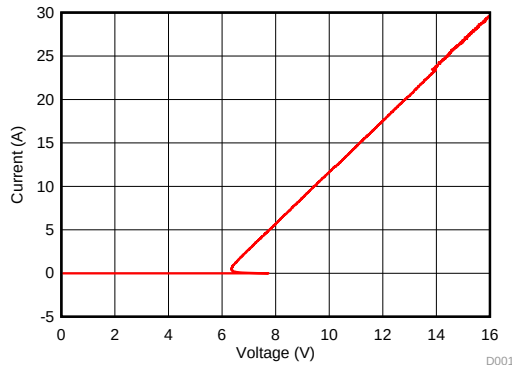
图 1. Positive TLP Curve, IO pin to GND ( t_p = 100 ns)
