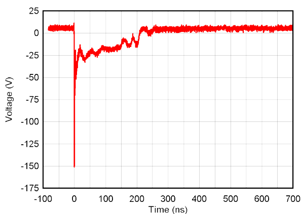
图 7-4. -8-kV Clamped IEC Waveform
