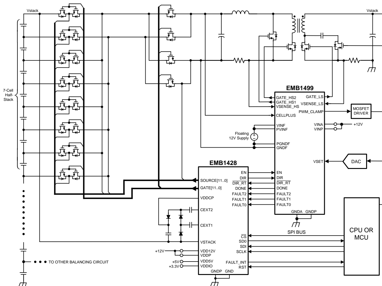
Figure 1. Typical Application
