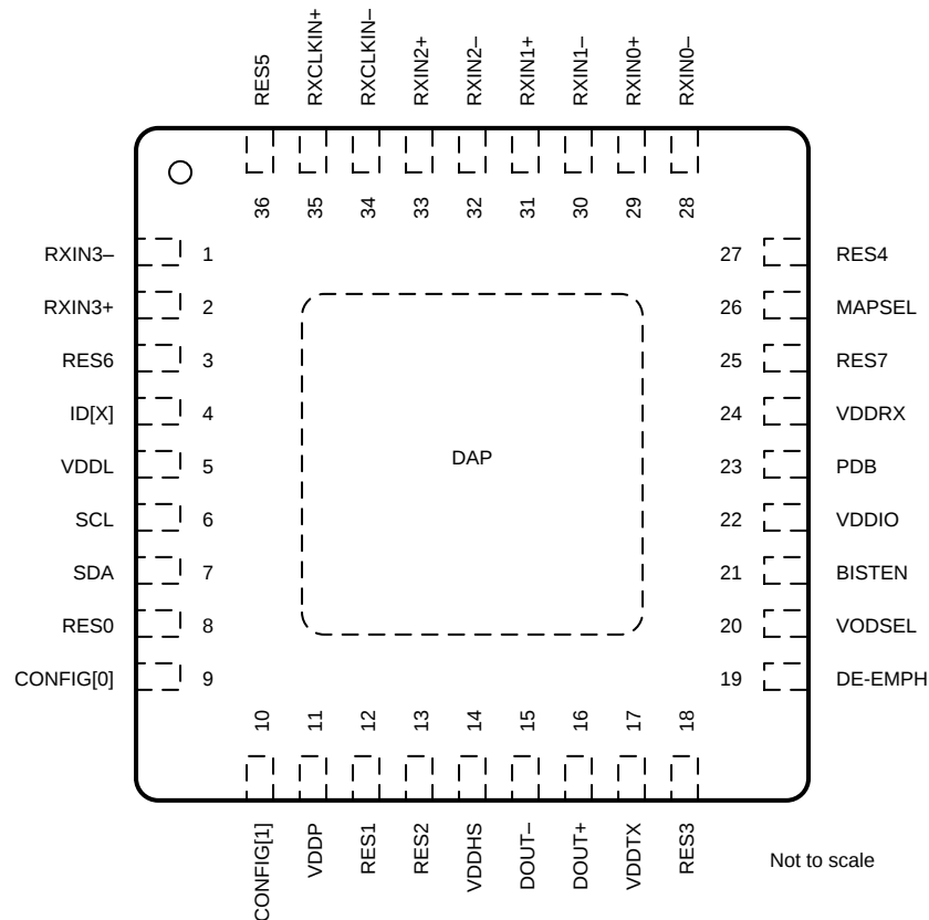
Pin Functions: DS92LV0421
