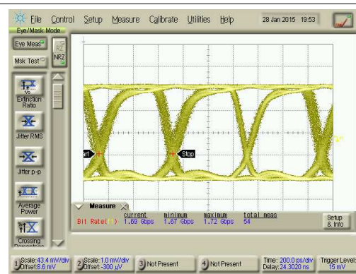
Figure 42. CMLOUT of Deserializer from 48-MHz Input Clock
