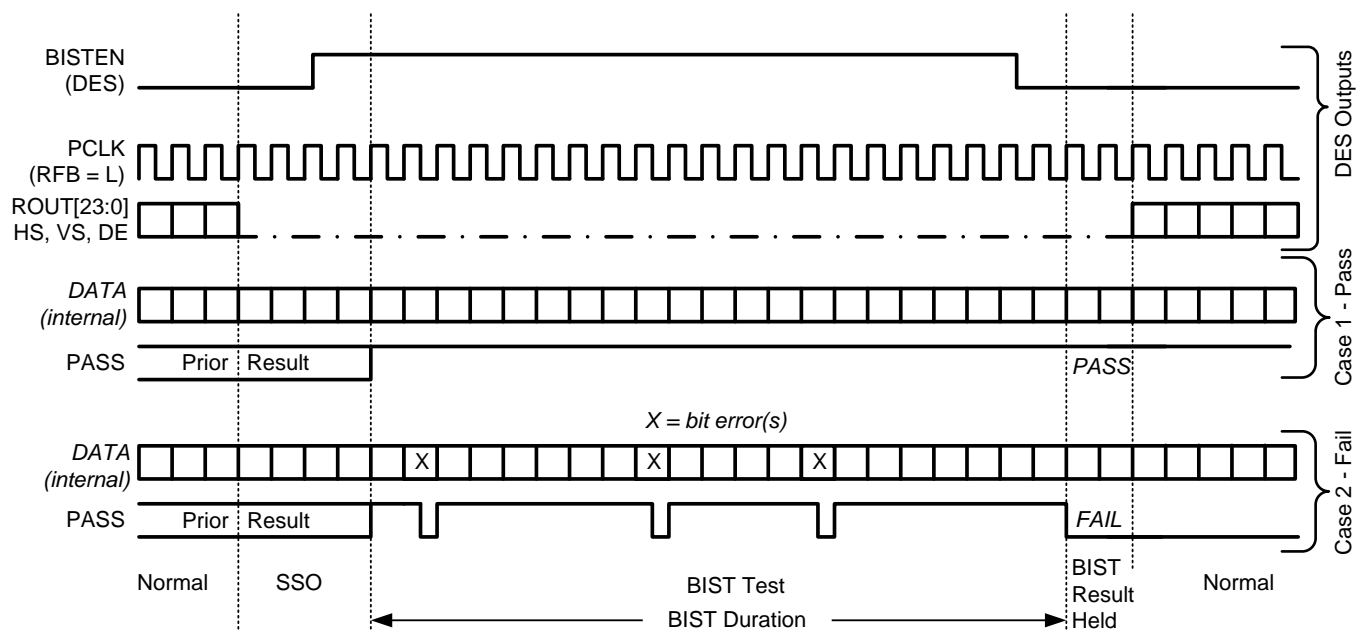
Figure 16. BIST Waveforms
