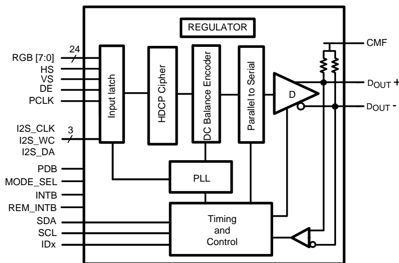
Figure 11. Block Diagram
