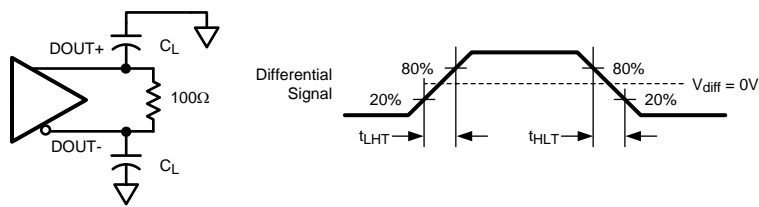
Figure 4. Serializer CML Output Load and Transition Time
