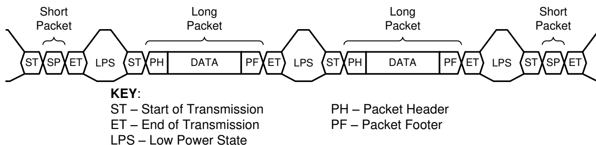
图 5-6. CSI-2 Protocol Layer With Short and Long Packets
