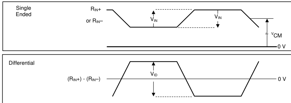
图 4-2. FPD-Link III Receiver V_{\text{ID}} , V_{\text{IN}} , V_{\text{CM}}
