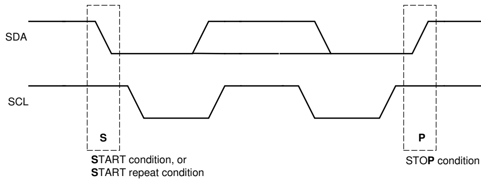
图 7-25. START and STOP Conditions
