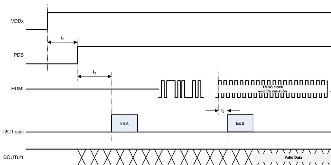
图 33. Initialization Sequencing
