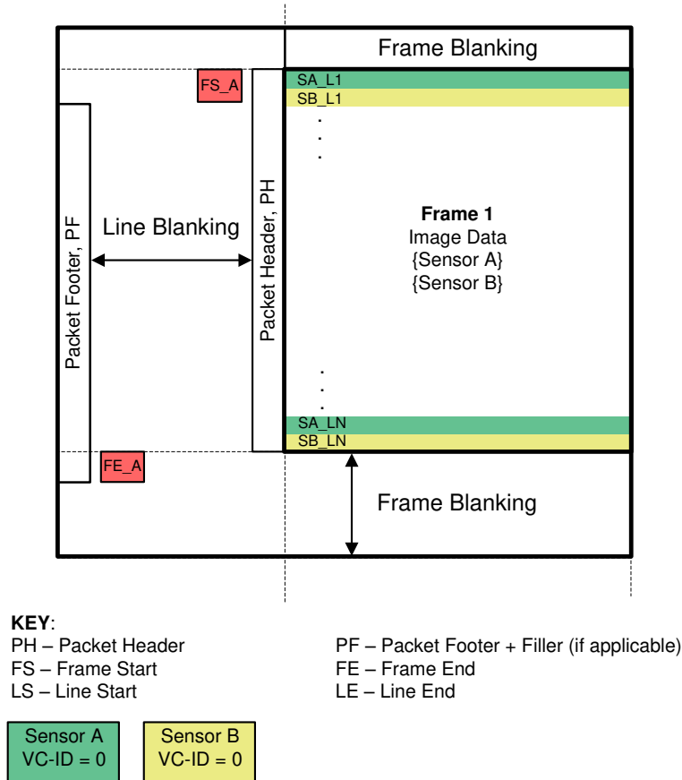
图 7-21. Line-Interleave Format
