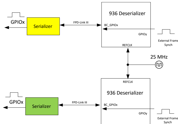
图 7-17. External FrameSync With Two DS90UB936 Deserializers
