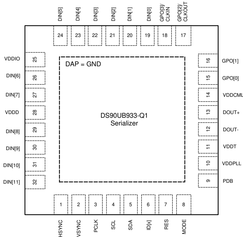
图 5-1. RTV Package 32-Pin WQFN Top View
