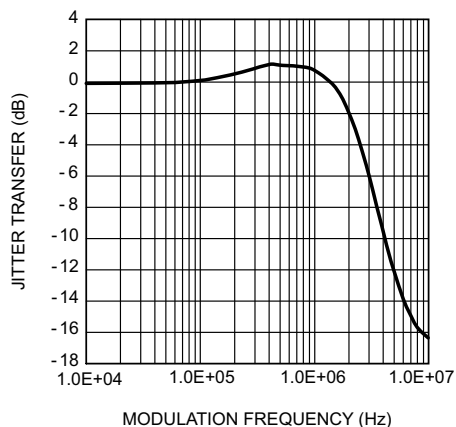
图 6-11. Typical Serializer Jitter Transfer Function
