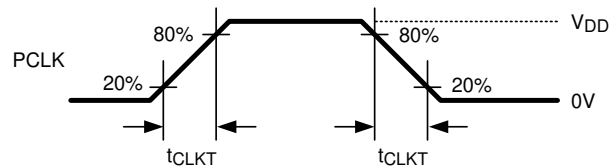
图 6-7. Serializer Input Clock Transition Times
