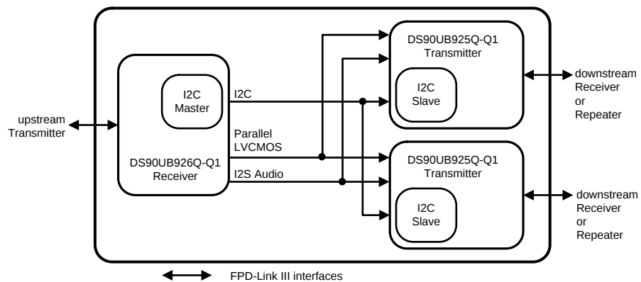
Figure 21. 1:2 Repeater Configuration
