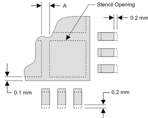
Figure 28. No Pullback WQFN, Single Row Reference Diagram
