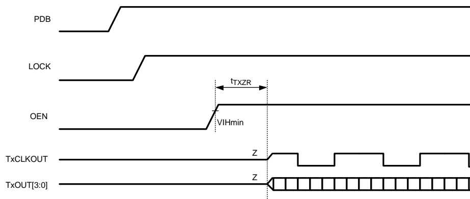
Figure 6. FPD-Link (OpenLDI) Outputs Enable Delay
