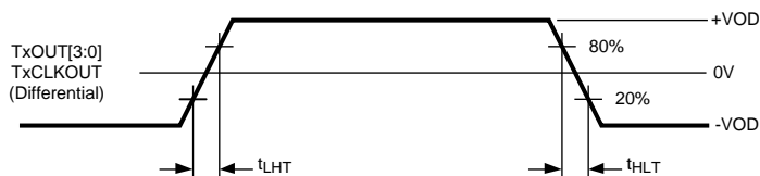
Figure 11. Input Transition Times
