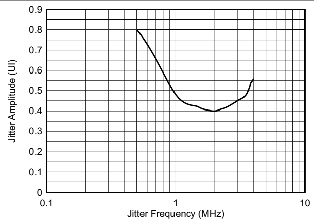
图 6-12. Typical System Input Jitter Tolerance Curve - DS90UB913A Linked to DS90UB914A
