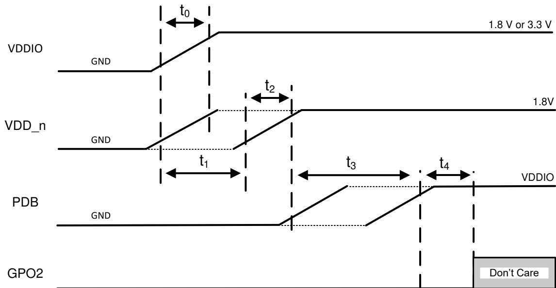
图 8-1. Suggested Power-Up Sequencing
