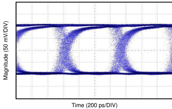
图 8-6. Coax Eye Diagram at 1.4-Gbps Line Rate (100-MHz Pixel Clock) from Deserializer CML Loop-through Output (CMLOUT±)
