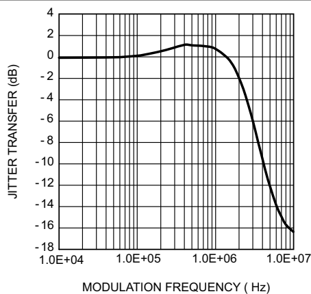
图 6-11. Typical Serializer Jitter Transfer Function
