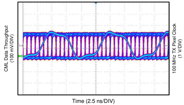
图 8-7. Coax Eye Diagram with 100-MHz TX Pixel Clock Overlay from Deserializer CML Loop-through Output (CMLOUT±)
