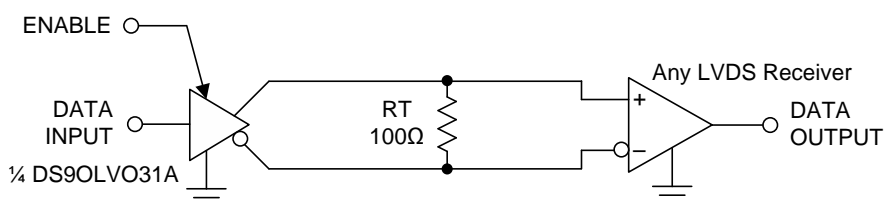
Figure 9. Point-to-Point Application
