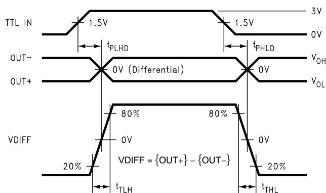
图 7-4. Differential Driver Propagation Delay and Transition Time Waveforms
