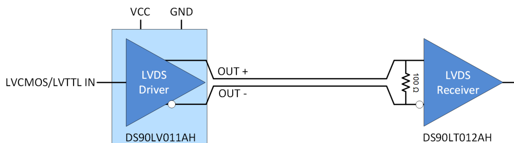
图 9-1. Point-to-Point Application
