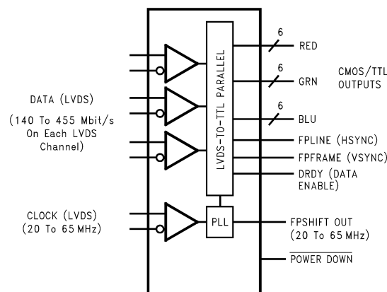
Figure 3. DS90CF364
