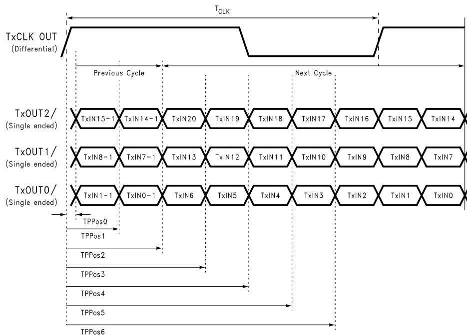
Figure 20. Transmitter LVDS Output Pulse Position Measurement
