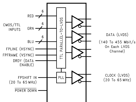
Figure 2. DS90C363
