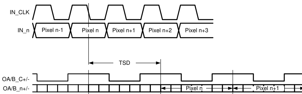
图 7-11. Single In, Single Out Mode Timing and Latency
