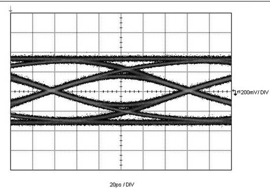
DS80PCI800 Settings: EQ[1:0] = [R, 1] or 0x0F, DEM[1:0] = [Float, Float] Figure 13. Test Setup 2, TL1 = 30-Inch 4-Mil FR4 Trace, TL2 = 15-Inch 4-Mil FR4 Trace
