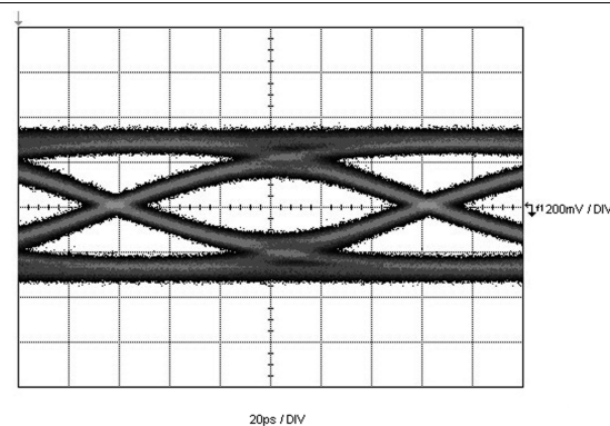
DS80PCI800 Settings: EQ[1:0] = [R, R] or 0x15, DEM[1:0] = [Float, Float] Figure 12. Test Setup 2, TL1 = 20-Inch 4-Mil FR4 Trace, TL2 = 15-Inch 4-Mil FR4 Trace
