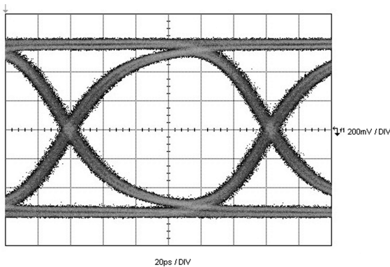
DS80PCI800 Settings: EQ[1:0] = [R, R] or 0x15, DEM[1:0] = [Float, Float] Figure 10. Test Setup 1, TL = 20-Inch 4-Mil FR4 Trace
