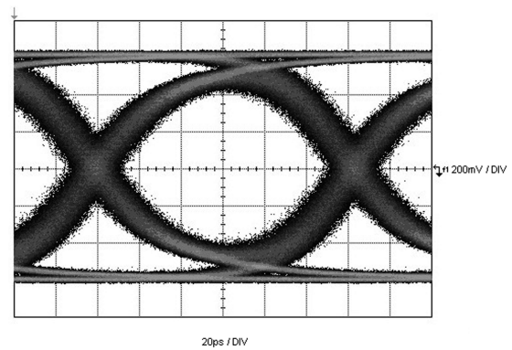
DS80PCI800 Settings: EQ[1:0] = [Float, R] or 0x1F, DEM[1:0] = [Float, Float] Figure 11. Test Setup 1, TL = 35-Inch 4-Mil FR4 Trace
