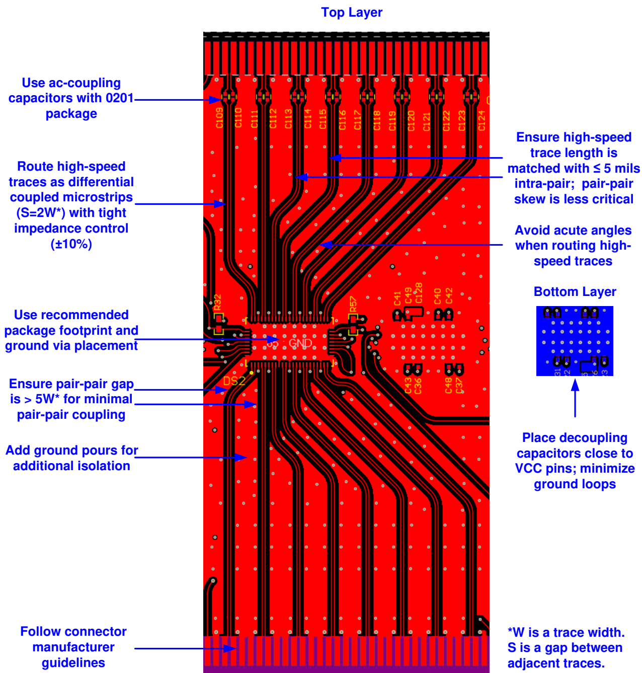
图 10-1. DS320PR822 Layout Example – Sub-Section of a PCIe Riser Card With CEM Connectors
