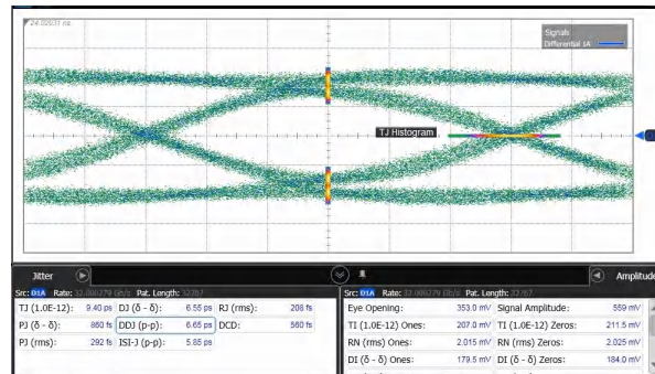
图 6-6. Through DS320PR 822 (7 dB Loss and DUT EQ = 0)
