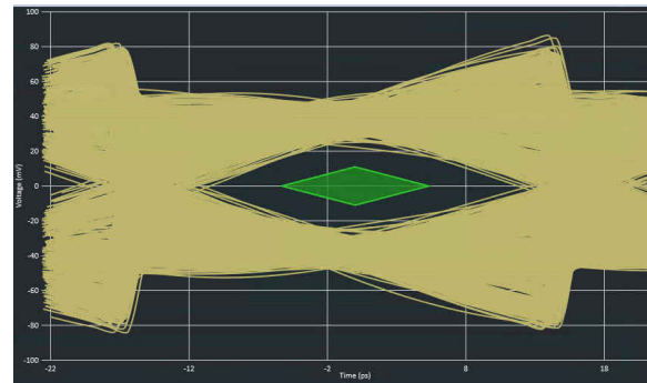
图 8-4. PCIe 5.0 link Baseline Setup Without Redriver Eye Diagram Using SigTest
