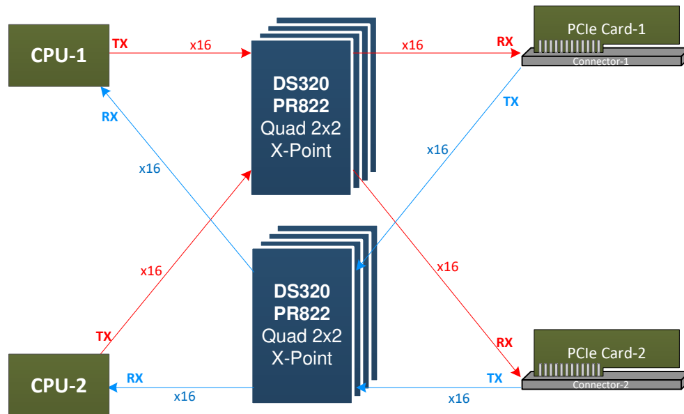
图 8-1. PCI Express x4 2x2 Cross-point Use Case Using DS320PR822
