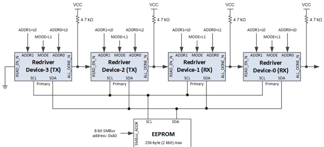
图 7-2. Daisy Chain Four DS320PR822 Devices to Read from Single EEPROM in 2x2 x8 Configuration
