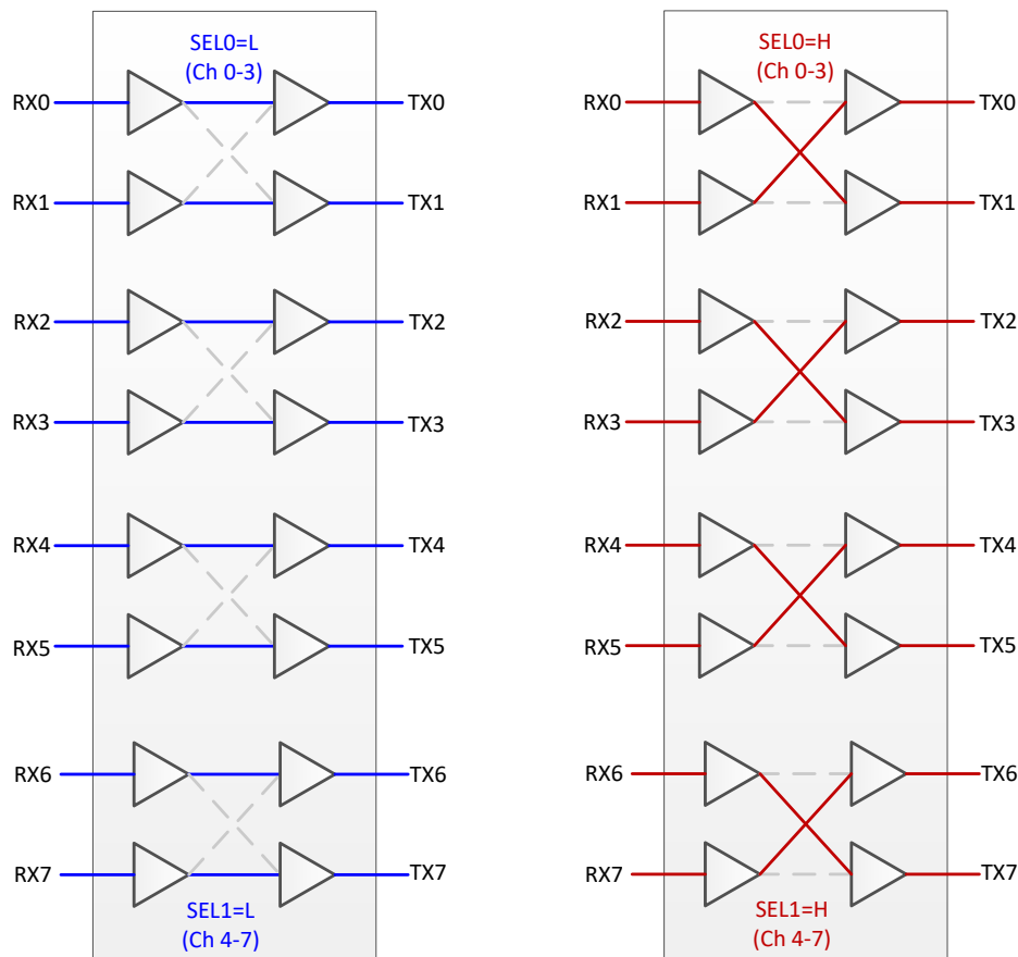
图 7-1. DS320822 Signal Flow Diagram for Cross-Point Mux Operation
