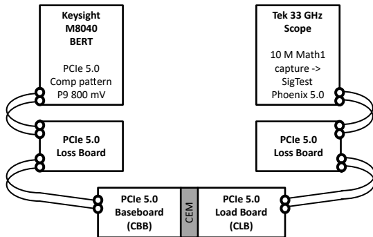
图 8-3. PCIe 5.0 Link Baseline Setup Without Redriver the Link Elements
