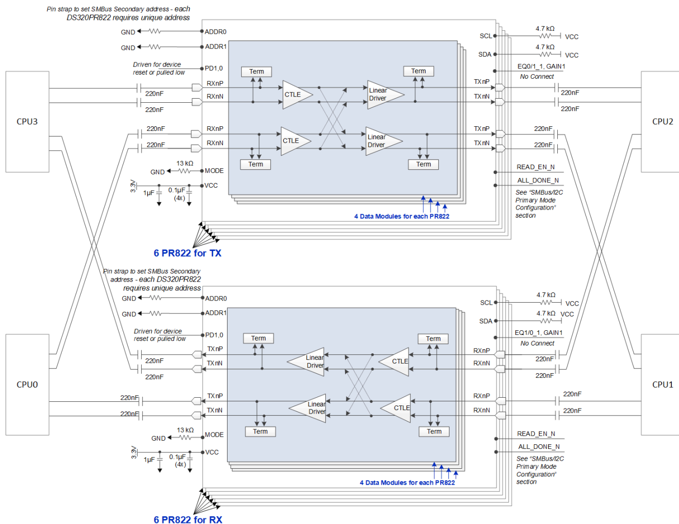
图 8-2. Simplified Schematic for UPI x24 Lane Configuration in SMBus/I 2 C Primary Mode
