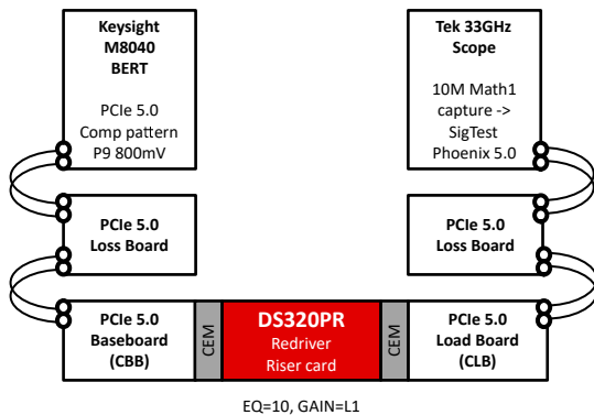
图 8-5. PCIe 5.0 Link Setup with the DS320PR822 the Link Elements
