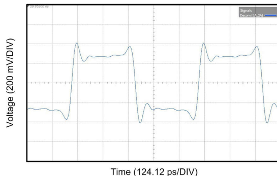
图 7-7. DS280DF810 FIR Transmit Equalization while Operating at 25.78125Gbps
