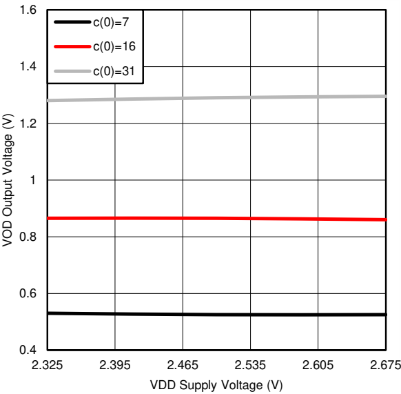
图 5-1. Typical VOD versus Supply Voltage
