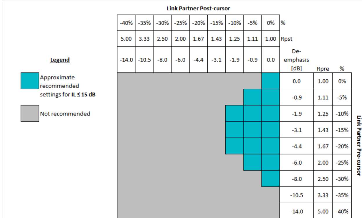
图 6-7. Guideline for Link partner FIR Settings When IL ≤ 15dB
