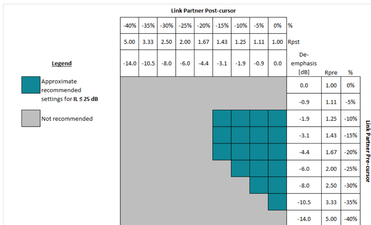
图 6-8. Guideline for Link partner FIR Settings When IL ≤ 25dB
