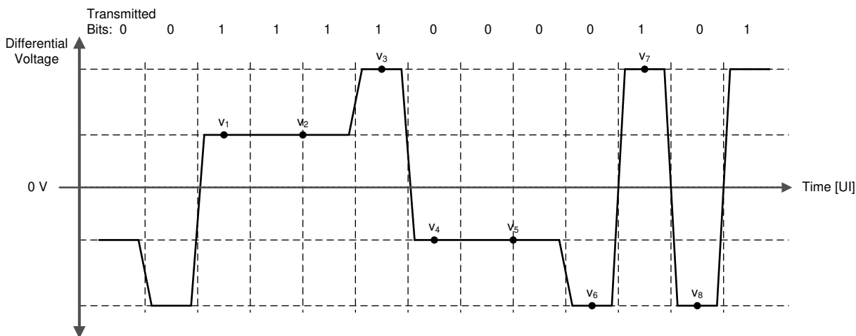
图 6-5. Conceptual FIR Waveform With Pre-Cursor Only
