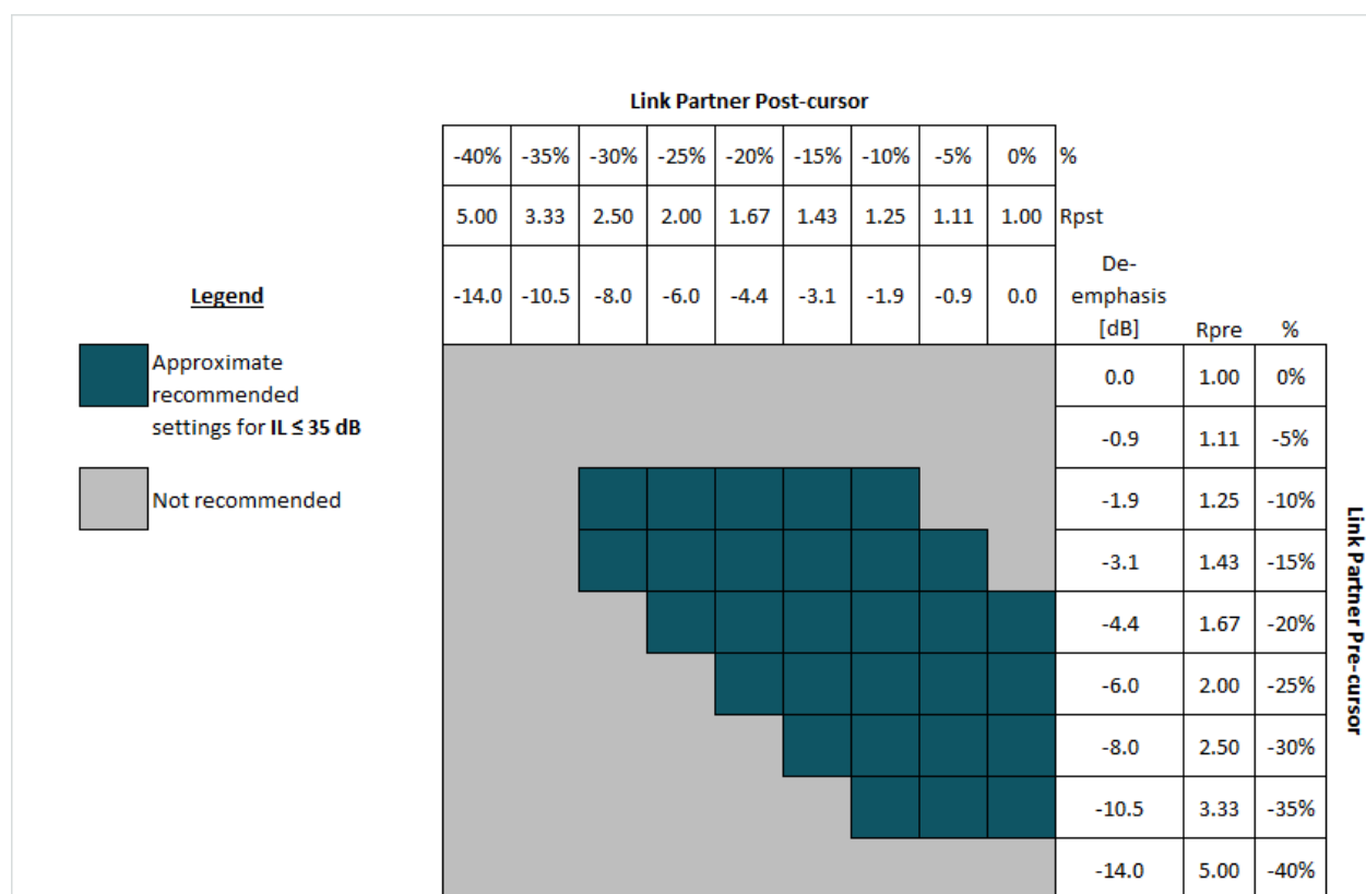
图 6-9. Guideline for Link partner FIR Settings When IL ≤ 35dB
