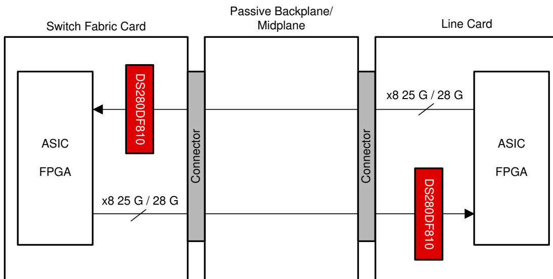
图 7-2. Backplane and Mid-Plane Application Block Diagram
