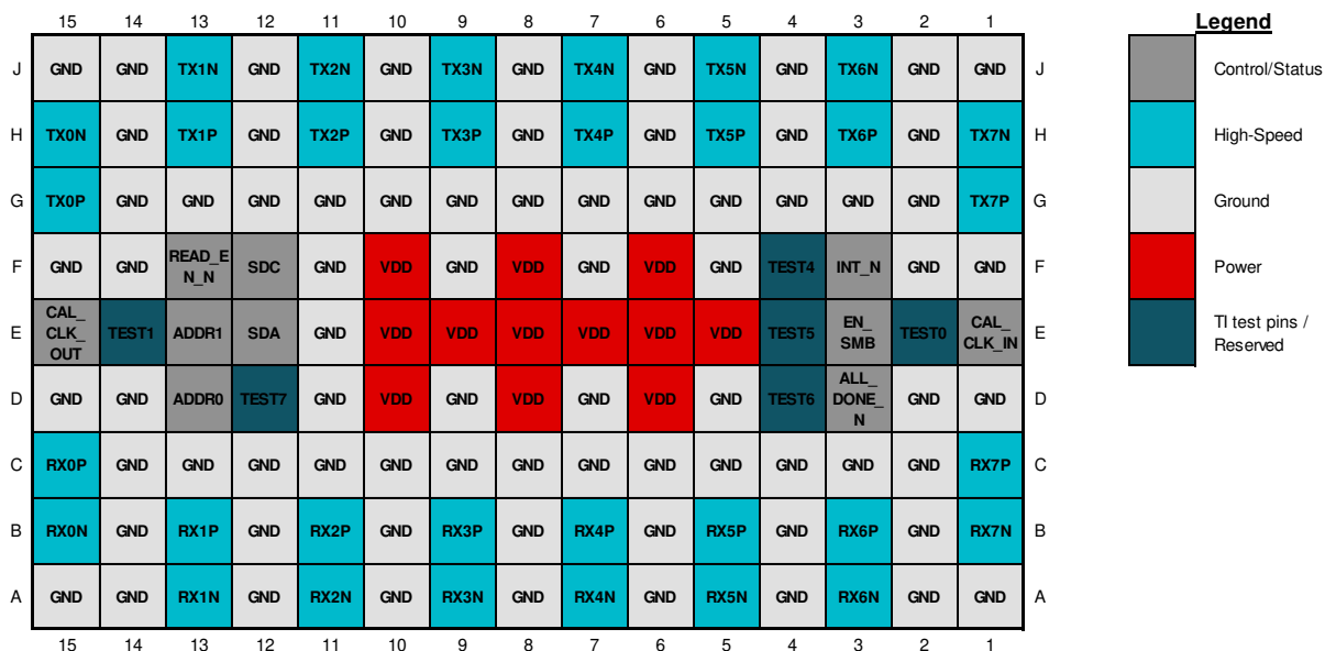
图 4-1. 135-Pin fcBGA, 0.8mm BGA Pin Pitch (Top View)
