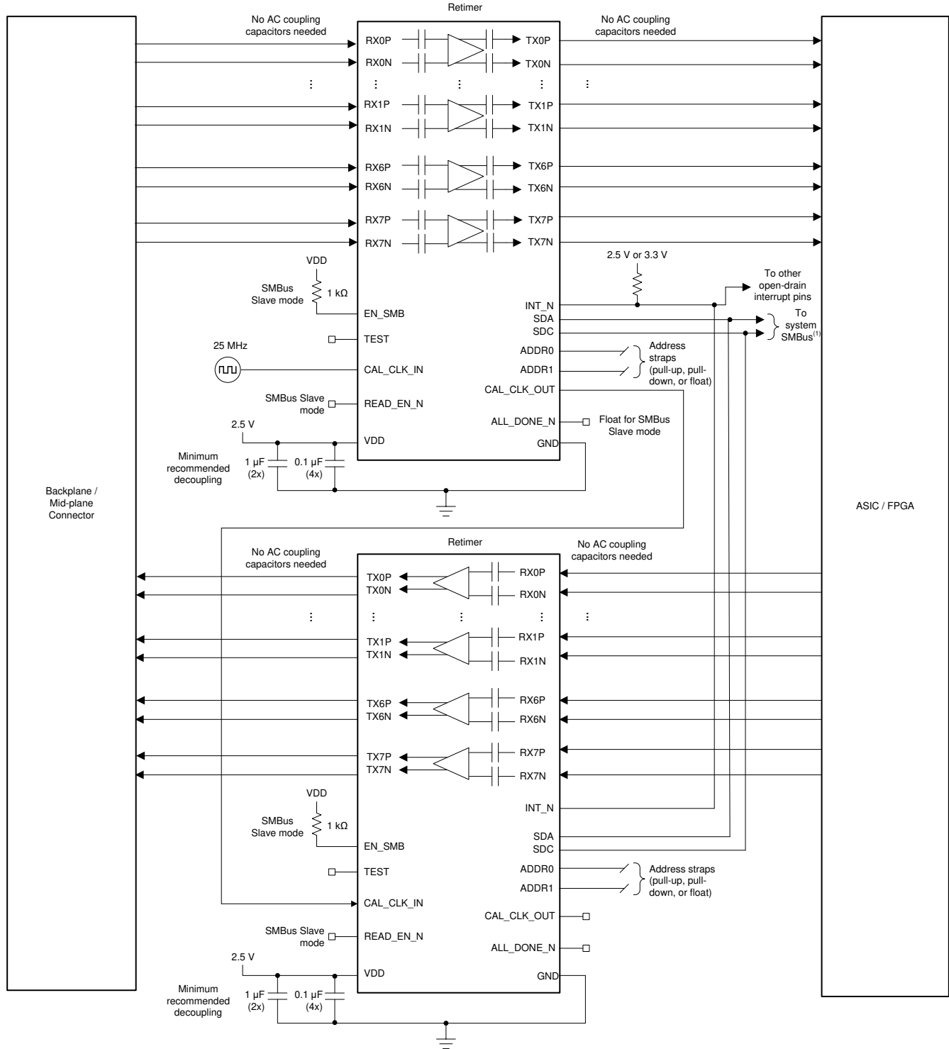
图 7-3. Backplane and Mid-Plane Application Schematic
