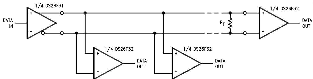
Figure 7. Typical Application
