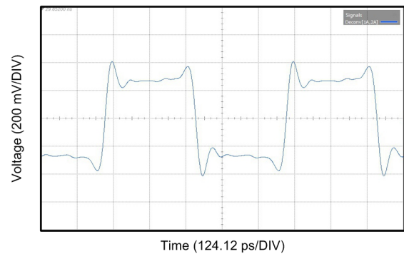
图 19. DS250DF410 FIR Transmit Equalization While Operating at 25.78125 Gbps
