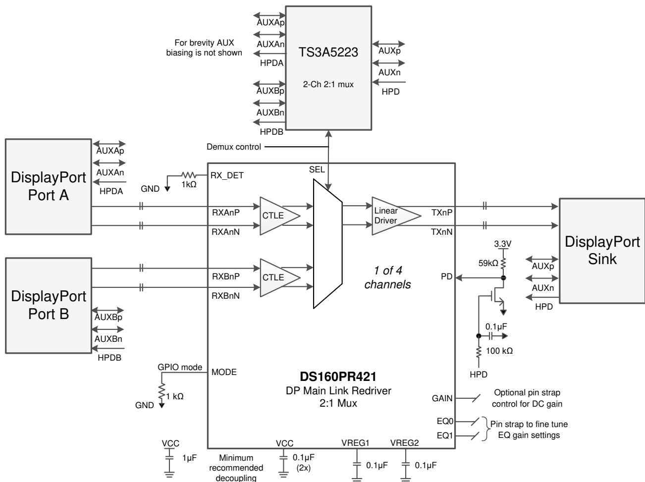
图 8-4. Simplified Schematic for DisplayPort Multiplexer Application
