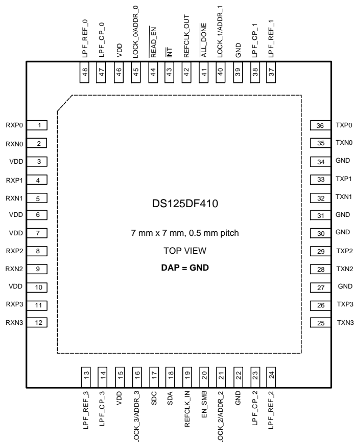
RHS Package 48-Pin WQFN Top View
