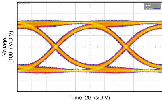
Figure 9. Typical Output Eye Diagram for the DS125DF410 Operating at 10.3125 Gbps with Default VOD of 600mVp-p and De-emphasis Setting of -2dB
