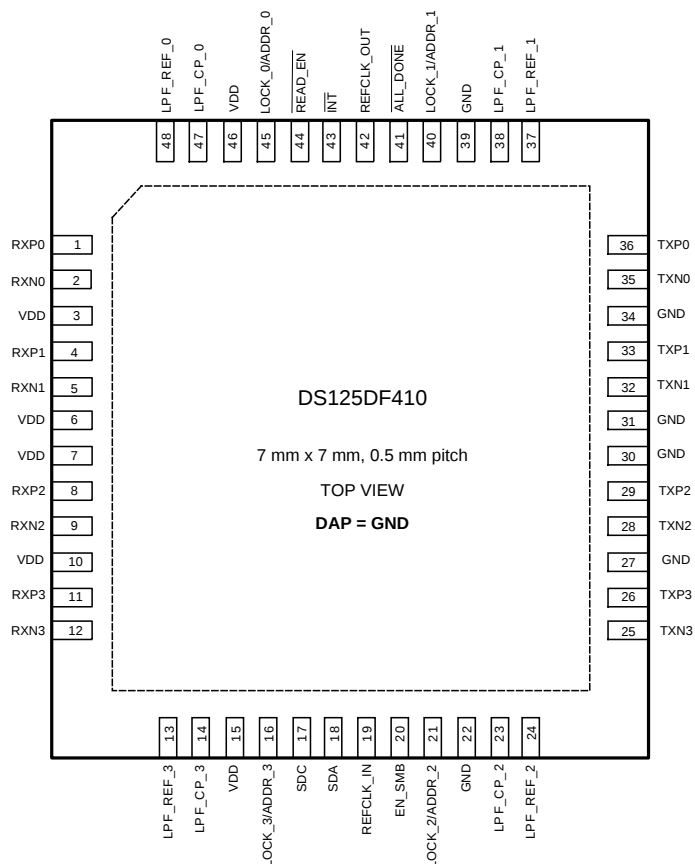
48-Pin WQFN Package RHS Top View
