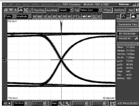
DS125BR401 settings: EQ[1:0] = 0, F = 0x02, DEM[1:0] = 0, 1 Figure 11. TL = 10-Inch 5-Mil FR4 Trace, 5 Gbps
