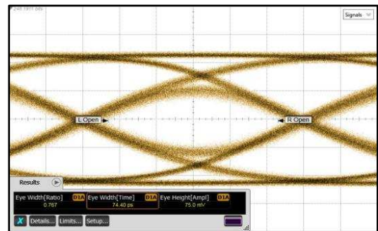
Figure 34. TL1 = 15 Inch 4-Mil FR4 Trace, TL2 = 10 Inch 4-Mil FR4 Trace, DS100BR111A CHA, 10.3125 Gbps
