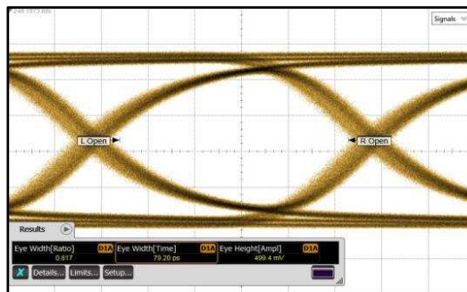
Figure 26. TL = 3-Meter 30-AWG 100 \Omega Twin-Axial Cable, DS100BR111A CHA, 10.3125 Gbps
