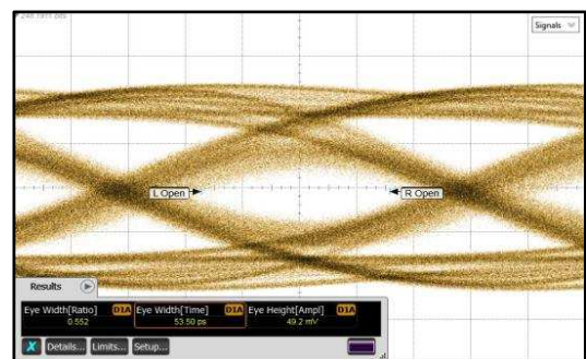
Figure 36. TL1 = 30 Inch 4-Mil FR4 Trace, TL2 = 10 Inch 4-Mil FR4 Trace, DS100BR111A CHA, 10.3125 Gbps
