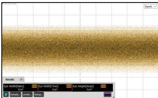
Figure 25. TL = 3-Meter 30-AWG 100 \Omega Twin-Axial Cable, No Repeater, 10.3125 Gbps
