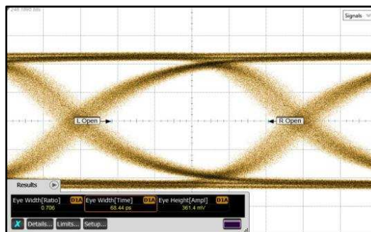
Figure 28. TL = 7-Meter 30-AWG 100 \Omega Twin-Axial Cable, DS100BR111A CHA, 10.3125 Gbps
