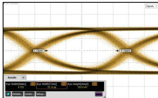
Figure 22. TL = 30 Inch 4-Mil FR4 Trace, DS100BR111 CHA, 10.3125 Gbps
