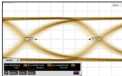
Figure 20. TL = 20 Inch 4-Mil FR4 Trace, DS100BR111 CHA, 10.3125 Gbps
