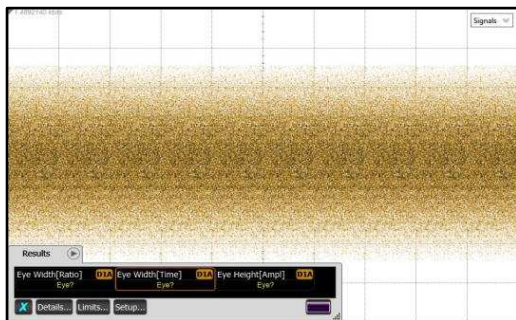
Figure 19. TL = 20 Inch 4-Mil FR4 Trace, No Repeater, 10.3125 Gbps
