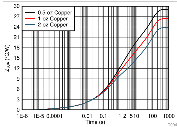
图 148. Transient Junction-to-Ambient Thermal Resistance ( Z_{\theta JA} ) vs Time for 4-Layer PCB with Copper-Pad Area of 4-cm 2
