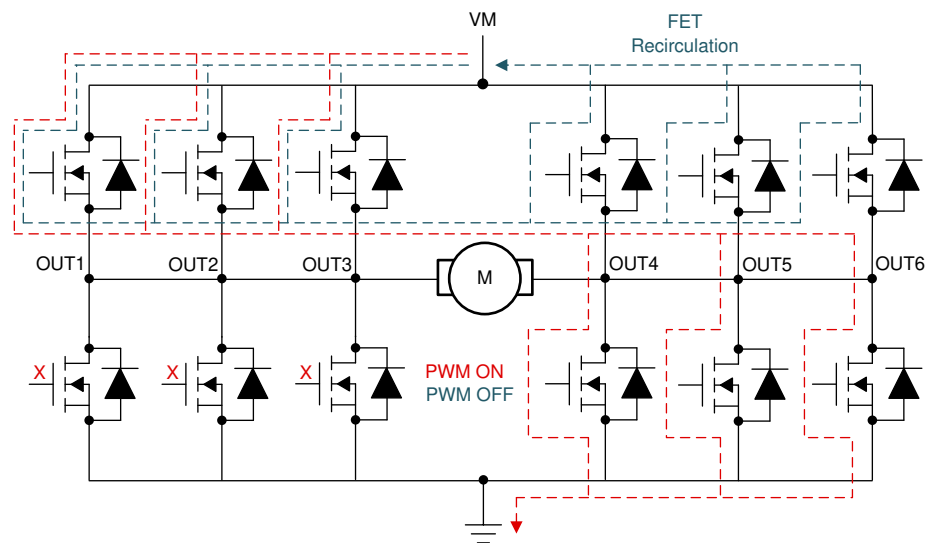
🔍 39. Parallel Mode (PWM with Synchronous Rectification = ON)
