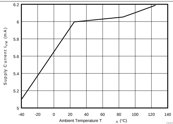
Figure 3. Supply Current over Temperature ( V_M = 24\text{ V} )
