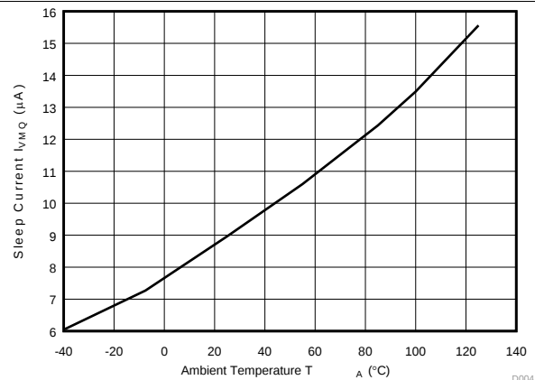
Figure 3. Supply Current over Temperature ( V_M = 24\text{ V} )
