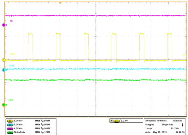
图 8-14. Driver Full On Operation With Current Chopping
