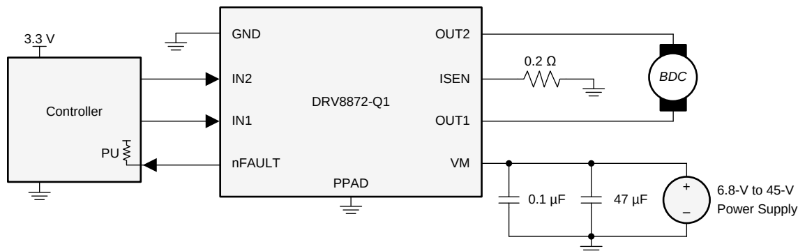
图 7. Typical Connections
