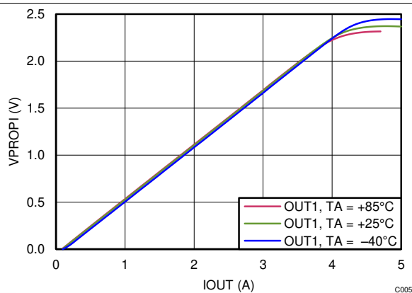
Figure 13. VPROPI Output, VCC = 4.2 V, OUT2 Overtemperature, 1 k \Omega
