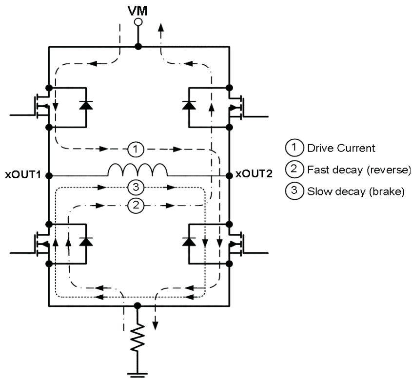
Figure 7. Decay Mode
