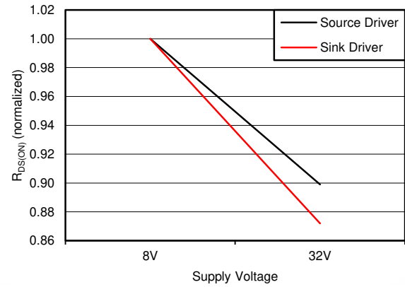
图 6-2. R_{DS(ON)} vs V_{BB} (Normalized to V_{BB} = 8 V)
