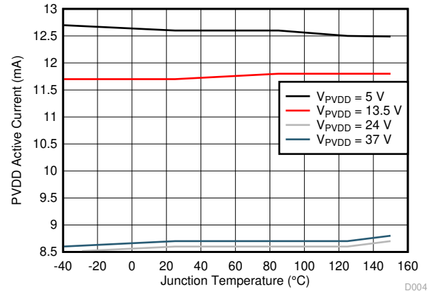
图 6-5. PVDD Active Current
