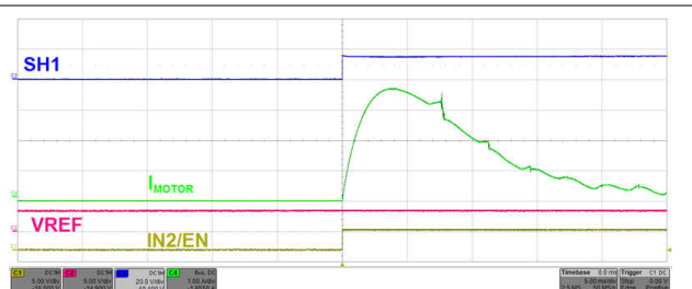
图 8-5. Current Profile on Motor Startup Without Regulation
