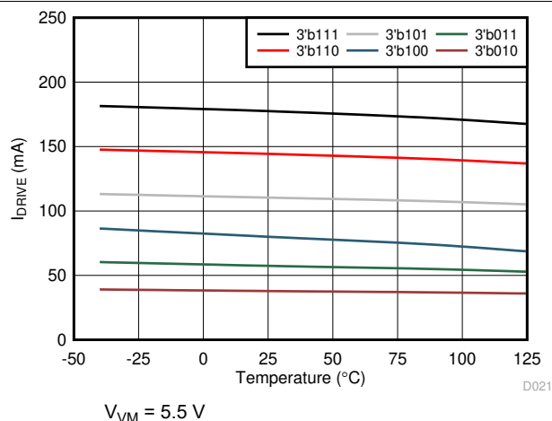
图 6-21. Low-Side Source Current
