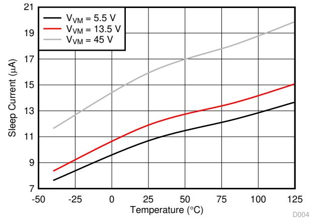
图 6-4. Sleep Current vs Temperature
