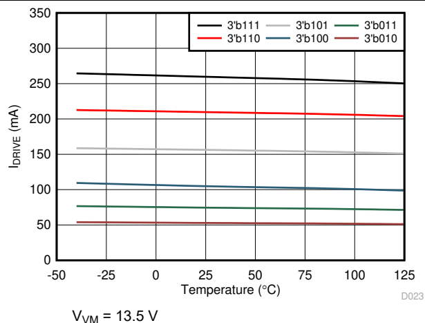
图 6-23. High-Side Source Current
