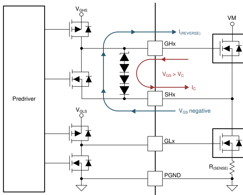
图 7-16. Gate Drive Clamp
