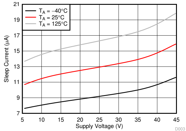
图 6-3. Sleep Current vs Supply Voltage (VM)
