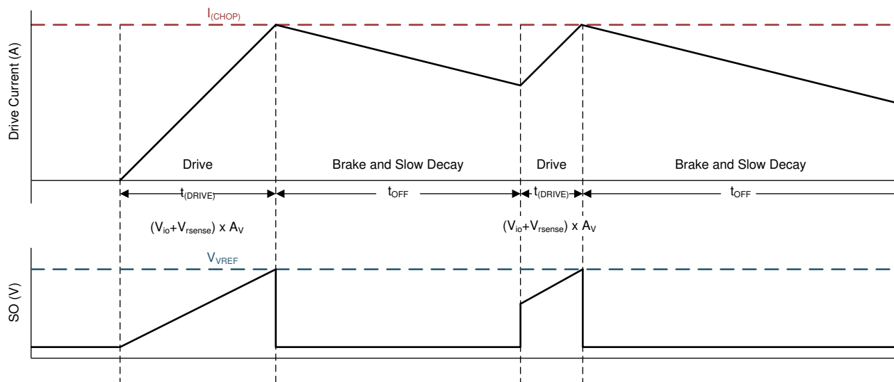
图 7-7. Current Sense Amplifier and Current Chopping Operation
