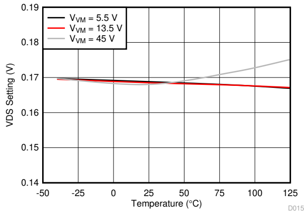
图 6-13. OCP Threshold Voltage
