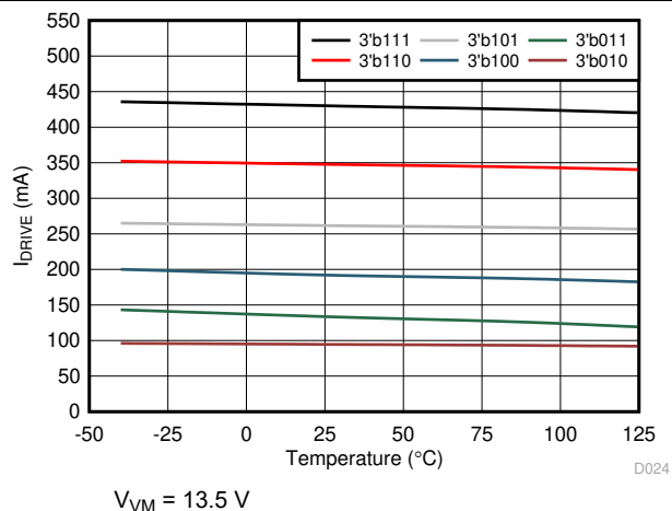
图 6-24. High-Side Sink Current
