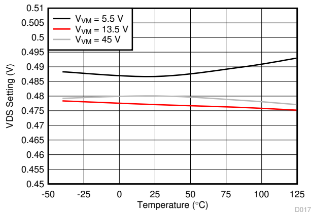
图 6-15. OCP Threshold Voltage
