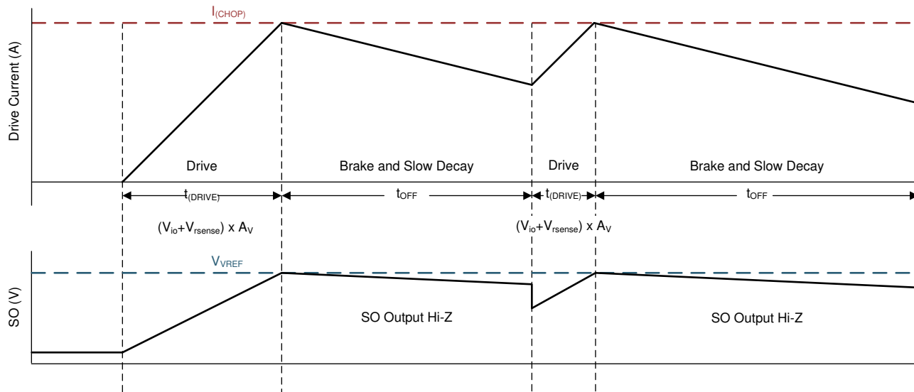
图 7-8. Sample and Hold Operation
