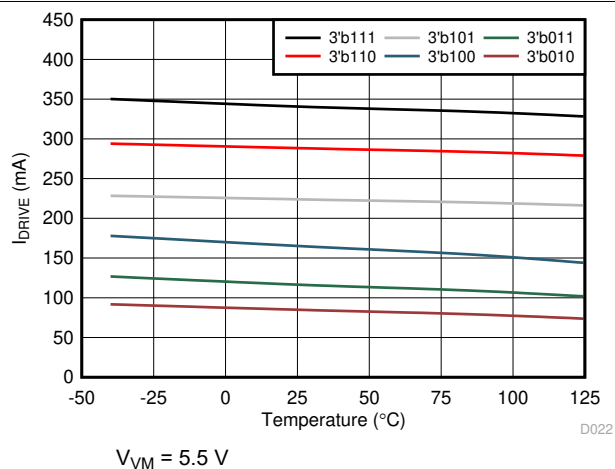
图 6-22. Low-Side Sink Current
