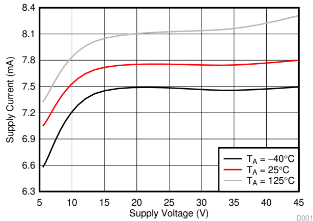
图 6-1. Supply Current vs Supply Voltage (VM)
