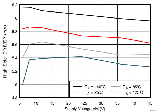
Figure 14. 6/12.5-mA High-Side IDRIVEP over VM
