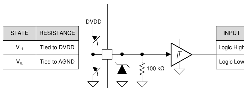
图 25. Logic-Level Input Pin Structure
