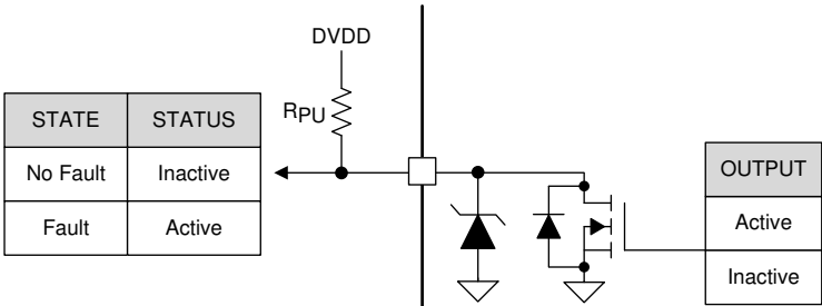
图 27. Open-Drain Output Pin Structure
