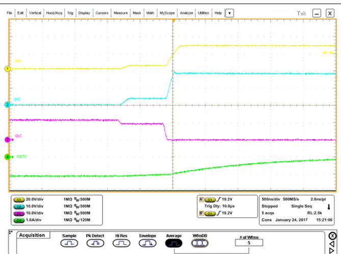
图 57. IDRIIVE Maximum Setting Negative Current
