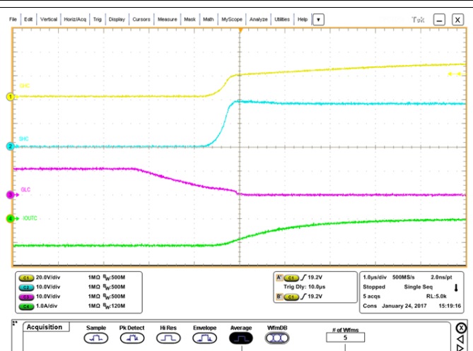
图 59. IDRIIVE Minimum Setting Negative Current
