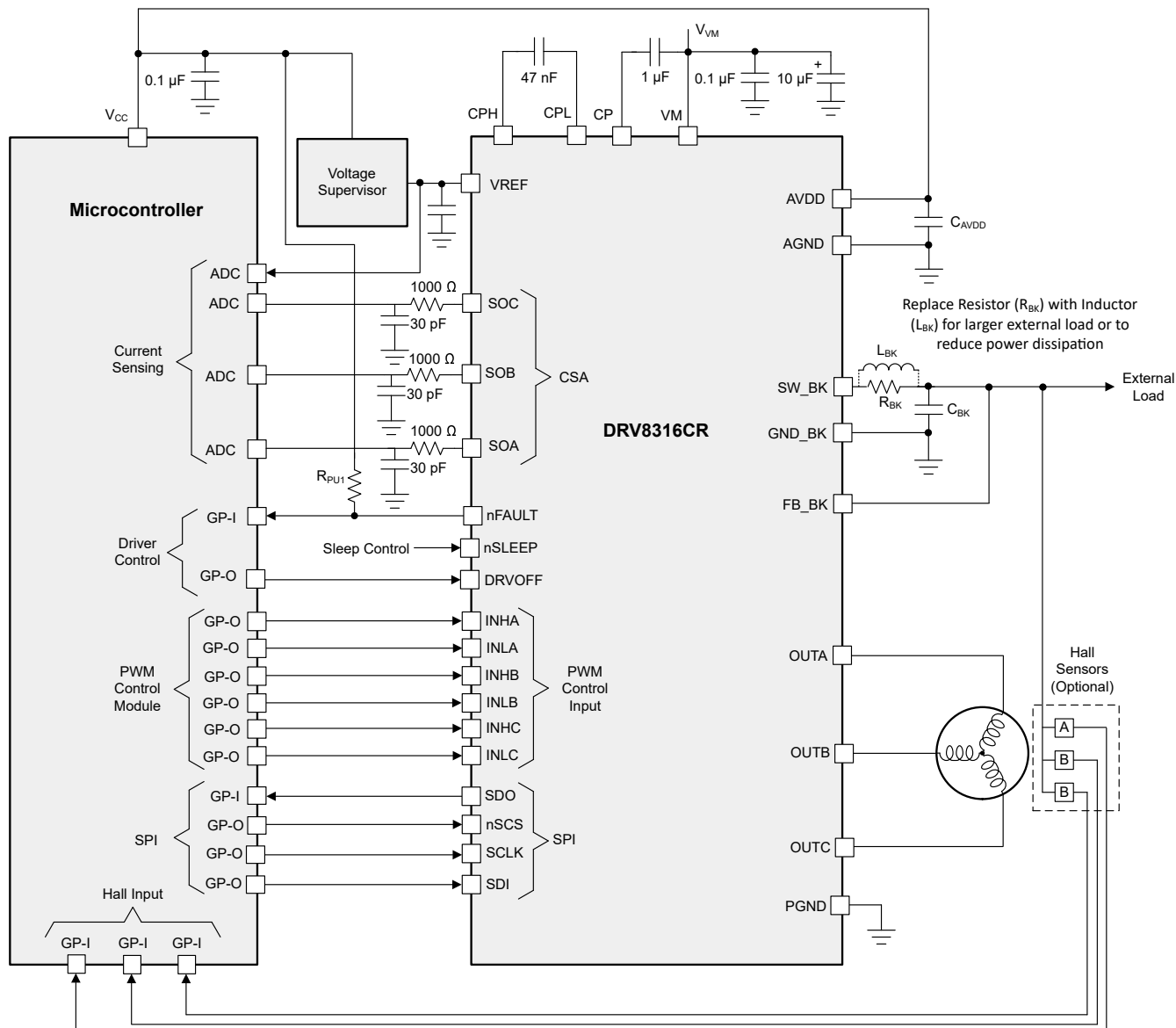
图 9-1. Primary Application Schematics
