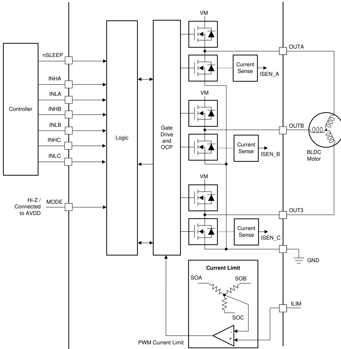
图 8-5. Current Limit Mode
