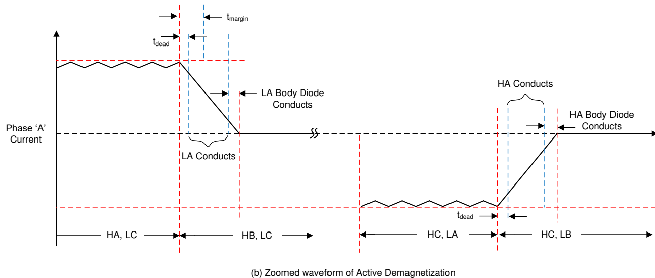
图 8-32. Current Waveforms for ASR in BLDC Motor Commutation
