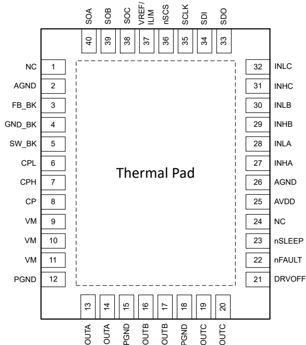
图 6-1. DRV8316R 40-Pin VQFN With Exposed Thermal Pad Top View
