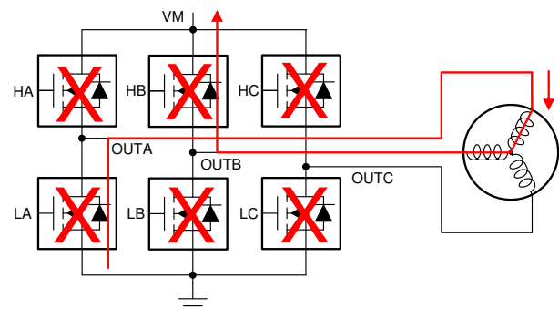
图 8-38. Coast State
