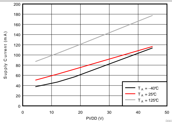
Figure 3. Standby Current
