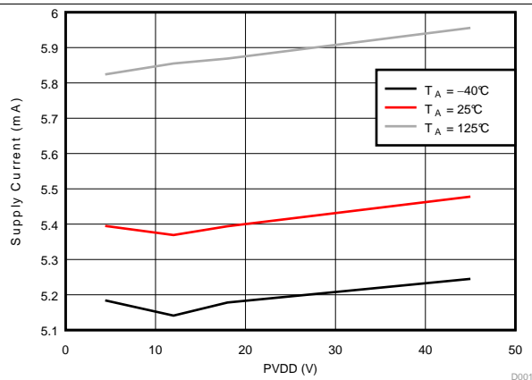
Figure 3. Standby Current
