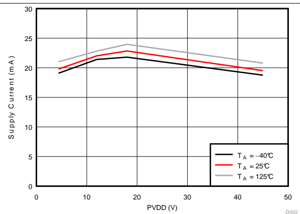
Figure 4. Operating Current
