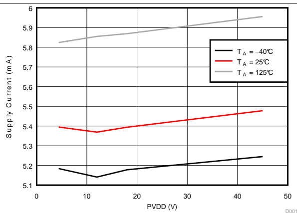
Figure 3. Standby Current
