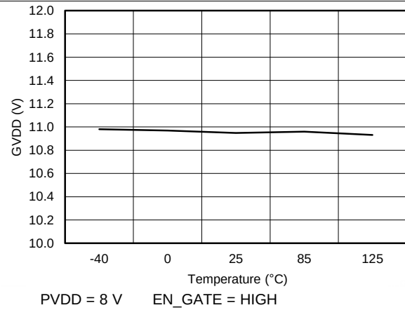
Figure 4. GVDD vs Temperature
