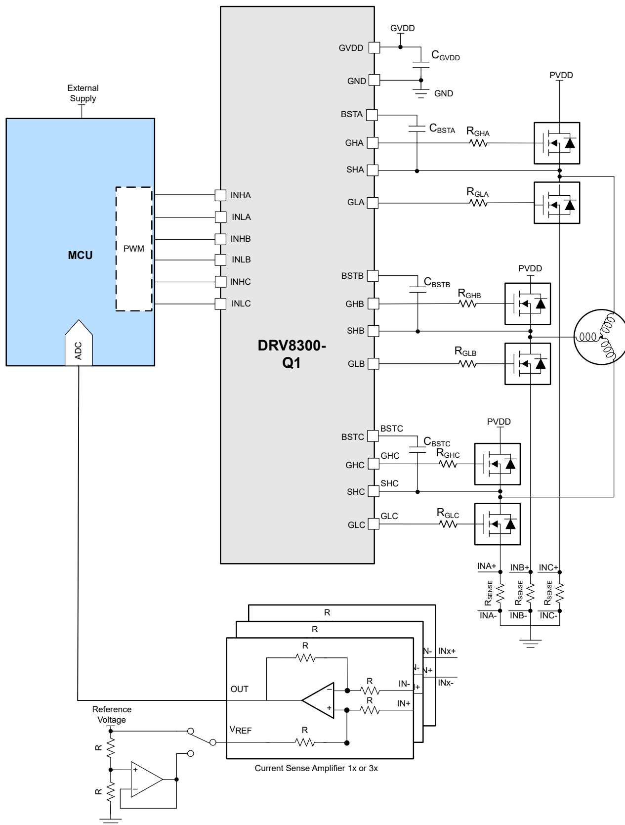
图 9-1. Application Schematic
